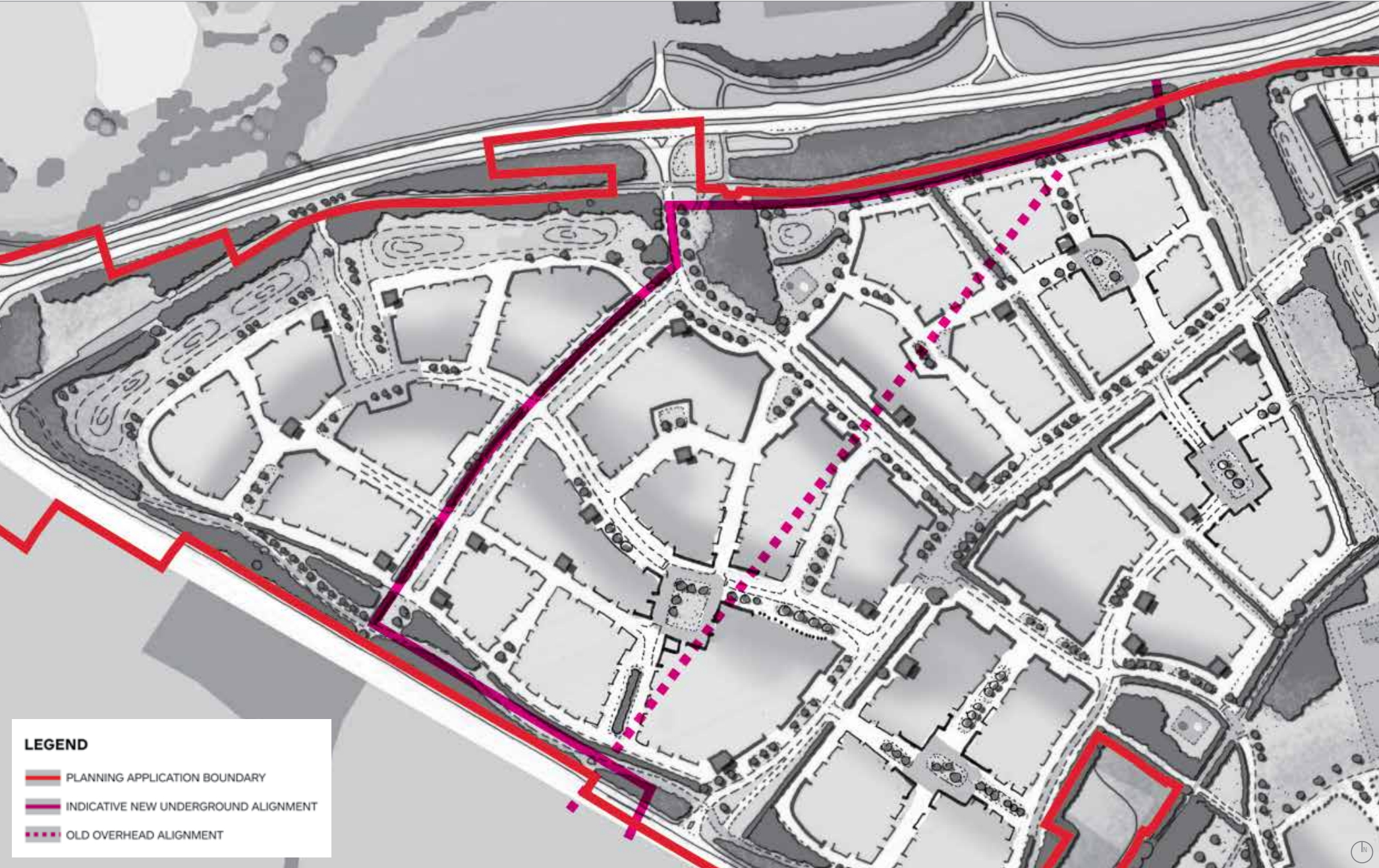
Figure 5.21: Proposed indicative alignment for undergrounding of high voltage powerlines
